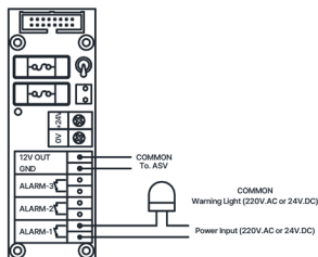
MAIN UNIT (SI-100IM)
