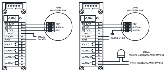
ALARM UNIT (SI-100IA)
