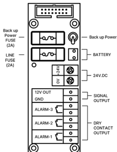
MAIN UNIT (SI-100IM)
