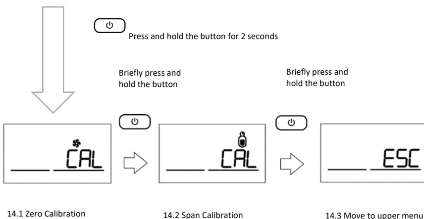
14. Calibration mode
