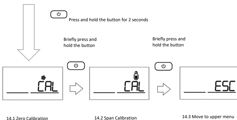
14. Calibration mode
