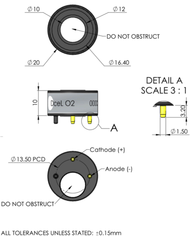
Product Dimensions in mm
